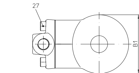
Fig. 634....2 (PN16/25) with screwed sockets - vertical installation
